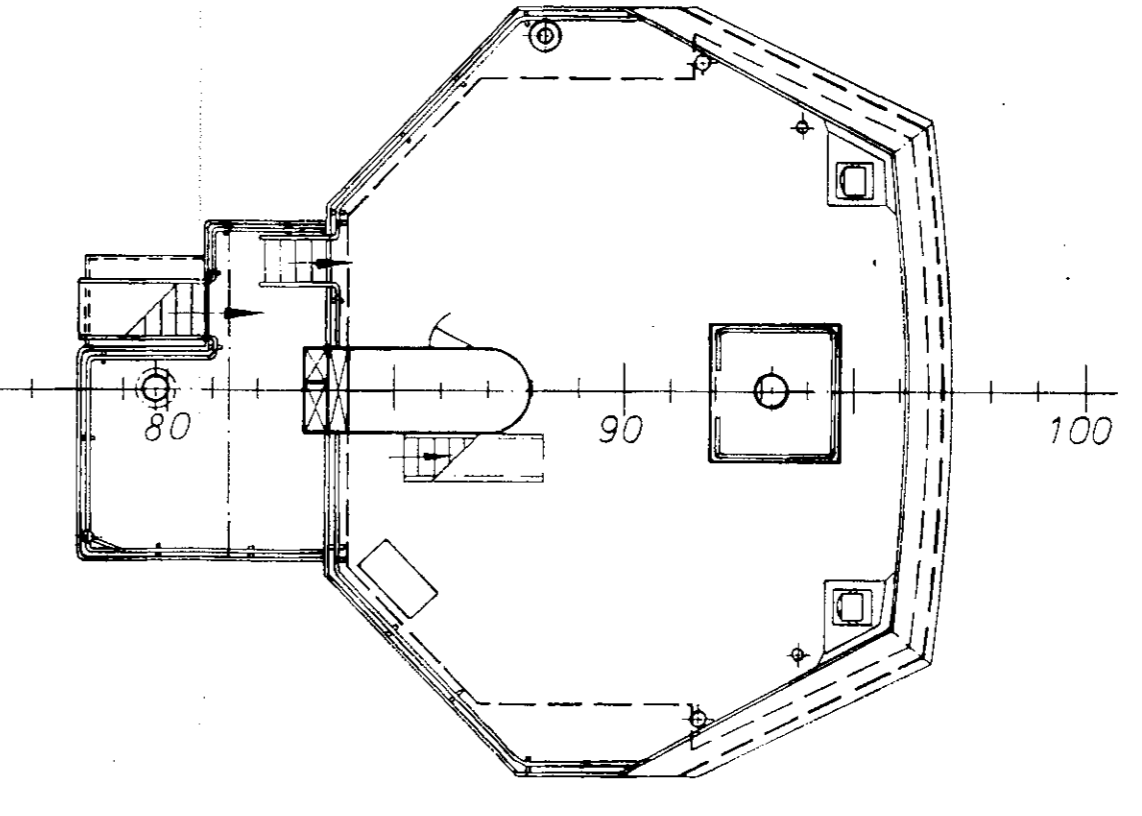
Peildeck
